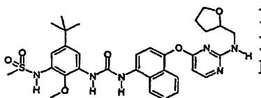
N-{5-tert-Butyl-2-methoxy-3-[3-(4-{2-[(tetrahydro-furan-2-ylmethyl)-amino]-pyrimidin-4-yloxy}-naphthalen-1-yl)-ureido]-phenyl}-methanesulfonamide;
